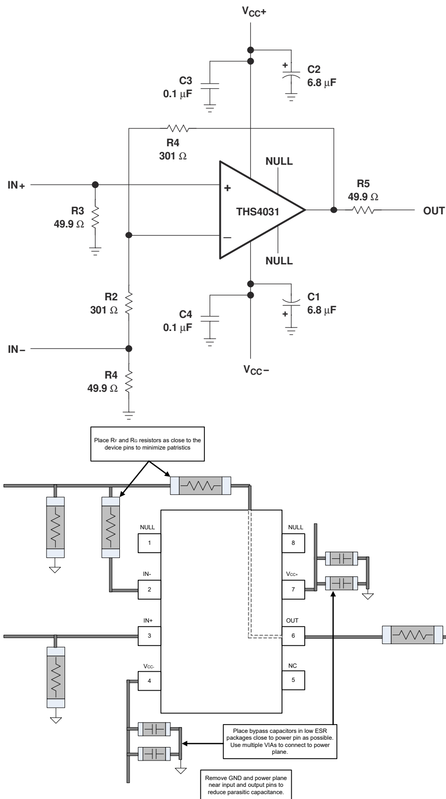
Figure 7-11. Layout Recommendations
