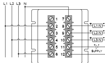
180-300 VL-L Connection
