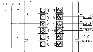
360-600 VL-L connection
