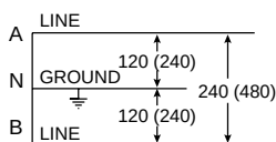
120/240 V, 3 W (240/480 V, 3 W) THREE-WIRE
