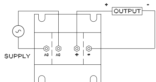
CR4340 100 - 600 Aac
