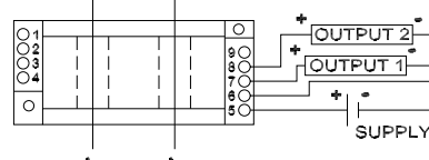
CR4160 Two Element 4 - 20 mA DC Output
