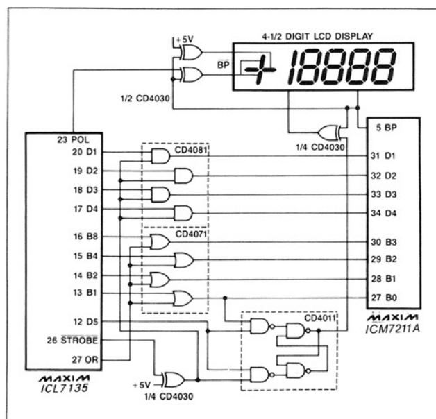
Figure 11. LCD Display with Digit Blanking on Overrange
