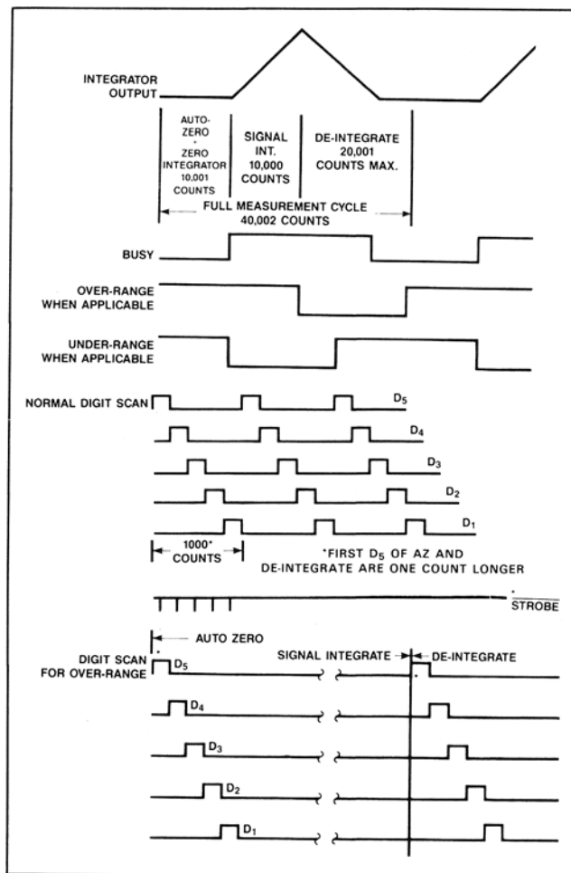
Figure 4. Timing Diagram
