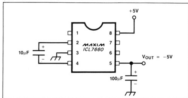
Figure 10A. Generating a Negative Supply
