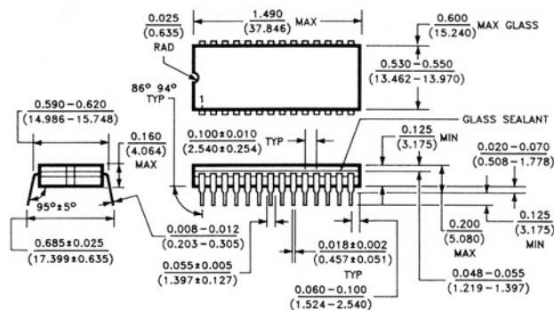
28 Lead Cerdip (JI) \theta_{JA} = 55^{\circ}\text{C/W}
