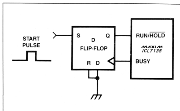
Figure 5. External RUN/HOLD Latch
