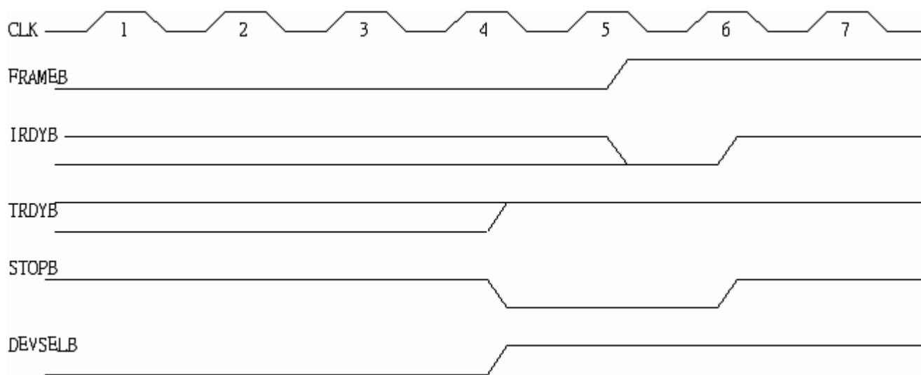
Figure 15. Target Initiated Termination - Abort
