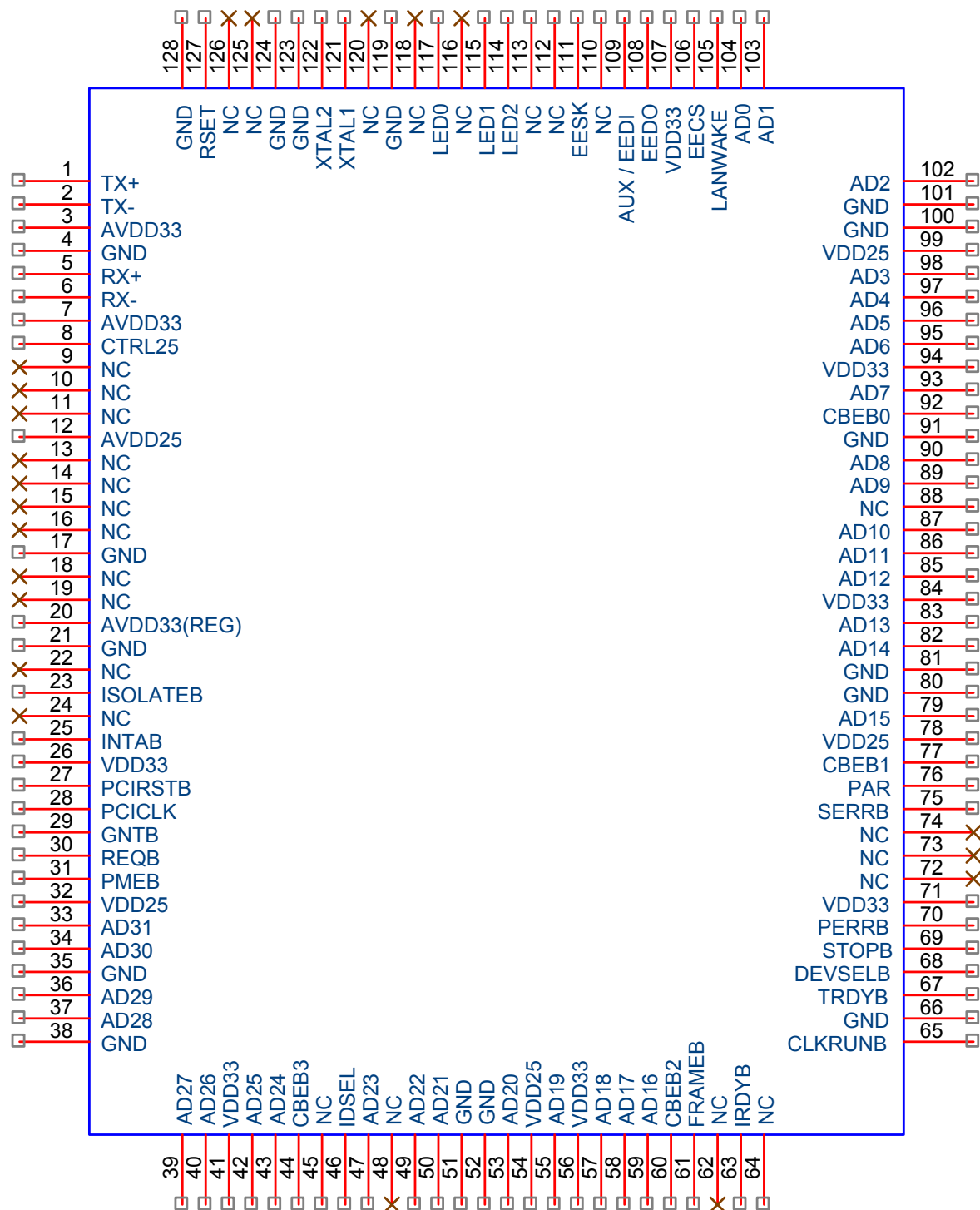
Figure 2. Pin Assignments
