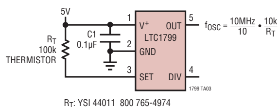
Temperature-to-Frequency Converter
