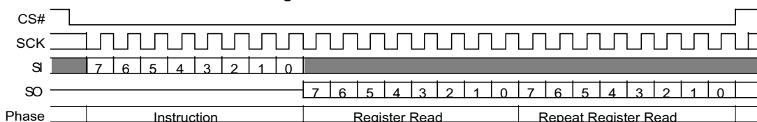
Figure 9.61 ASPRD Command
