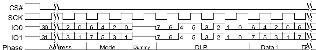
Figure 9.45 Continuous DDR Dual I/O Read Subsequent Access (4-Byte Address, EHPLC= 01b)
