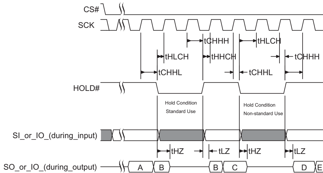
Figure 5.12 Hold Timing
