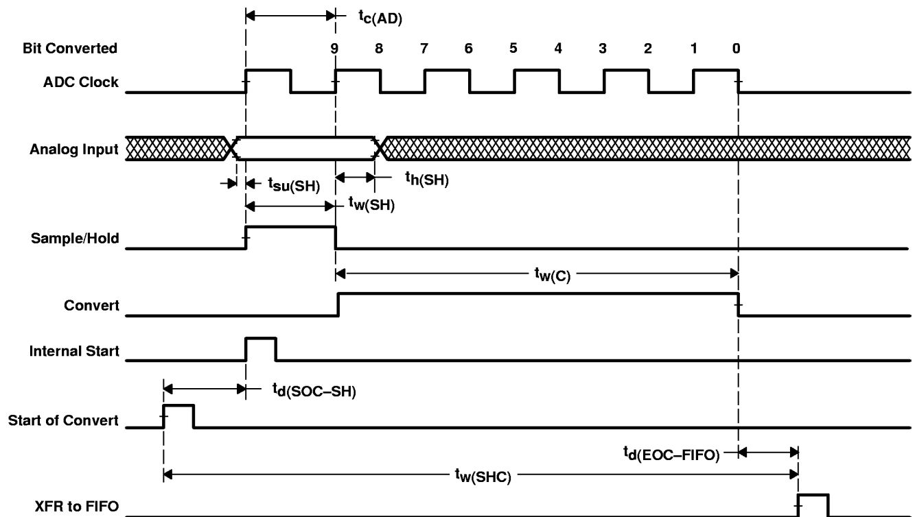
Figure 48. Analog-to-Digital Timing
