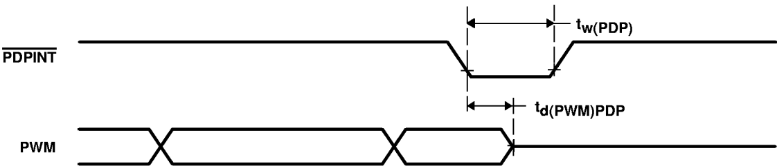
Figure 39. Power-Drive Protection Interrupt Timings
