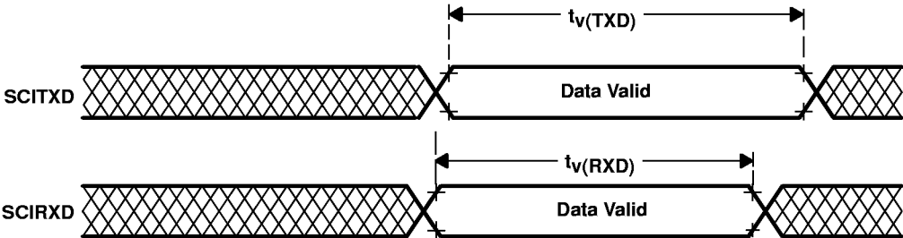
Figure 42. SCI Timings
