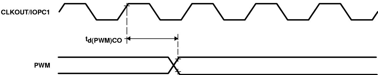
Figure 34. PWM and Compare Output Timings
