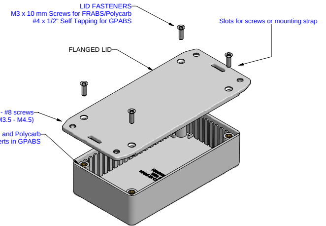
EXPLODED VIEW OF ENCLOSURE
