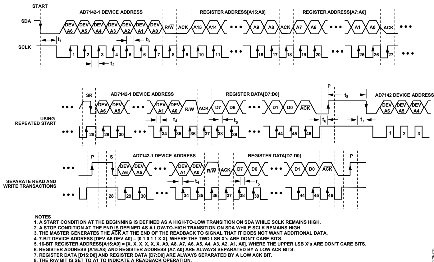
Figure 51. Example of I 2 C Timing for Single Register Readback Operation
