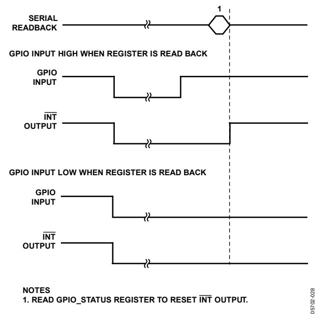
Figure 41. INT Output Controlled by the GPIO Input Example, GPIO_SETUP = 01, GPIO_INPUT_CONFIG = 00
