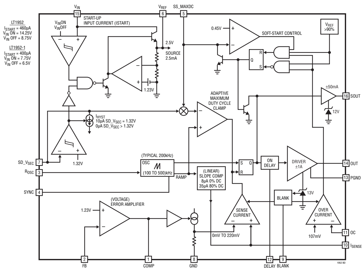
Figure 2. Block Diagram
