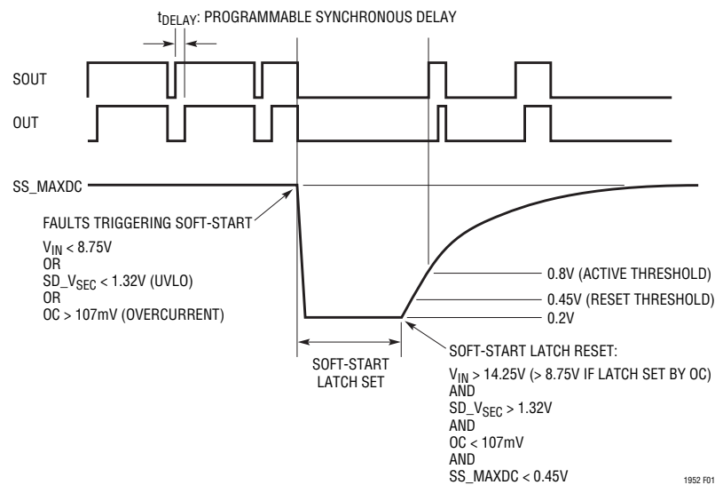
Figure 1. Timing Diagram
