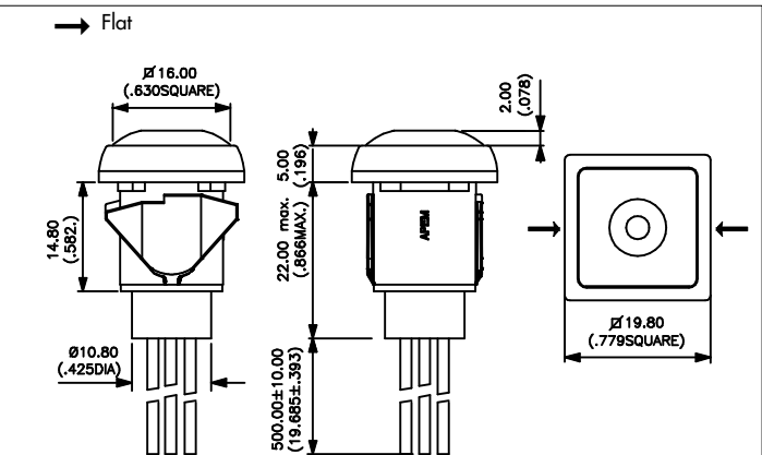
Normally Open
