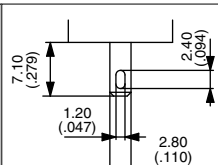
Quick-connect Z
