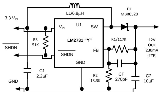
Figure 36. VIN = 3.3 V, VOUT = 12 V at 230 mA
