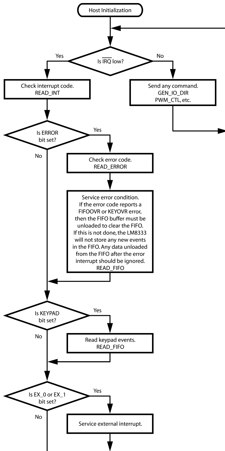
Figure 13. Interrupt Processing
