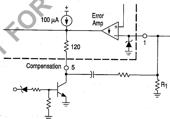
Figure 16. Over Voltage Shutdown Circuit
