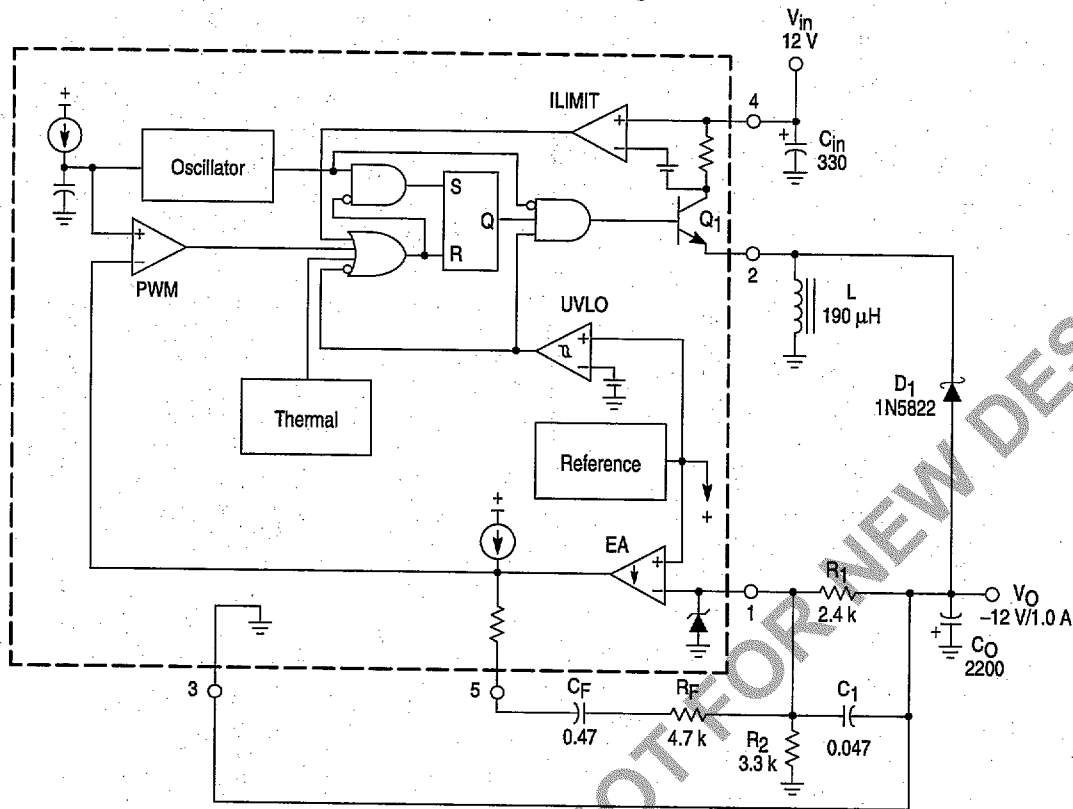
Figure 22. Voltage-Inverting Converter
