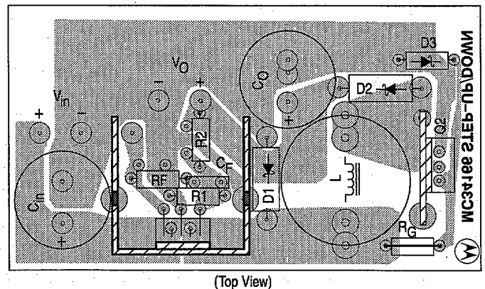
Figure 21. Step-Up/Down Converter Printed Circuit Board and Component Layout
