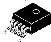
D2T SUFFIX PLASTIC PACKAGE CASE 936A (D2PAK)
