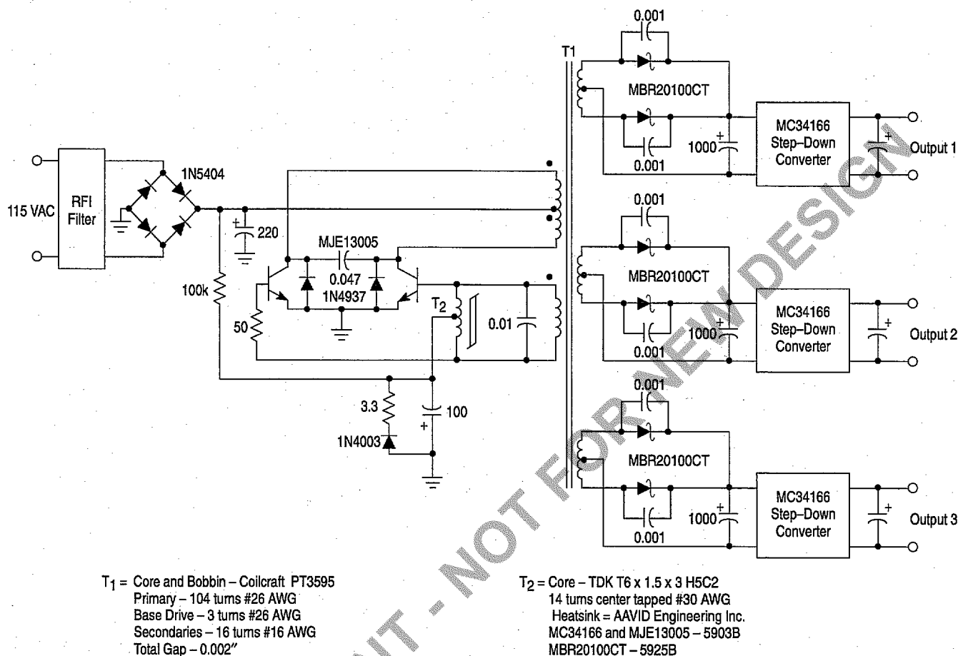
Figure 27. Off-Line Preconverter
