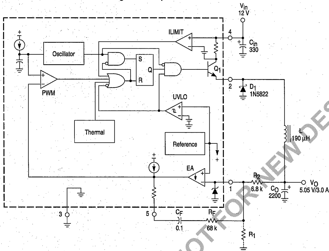
Figure 18. Step-Down Converter
