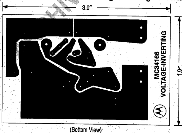
Figure 23. Voltage-Inverting Converter Printed Circuit Board and Component Layout
