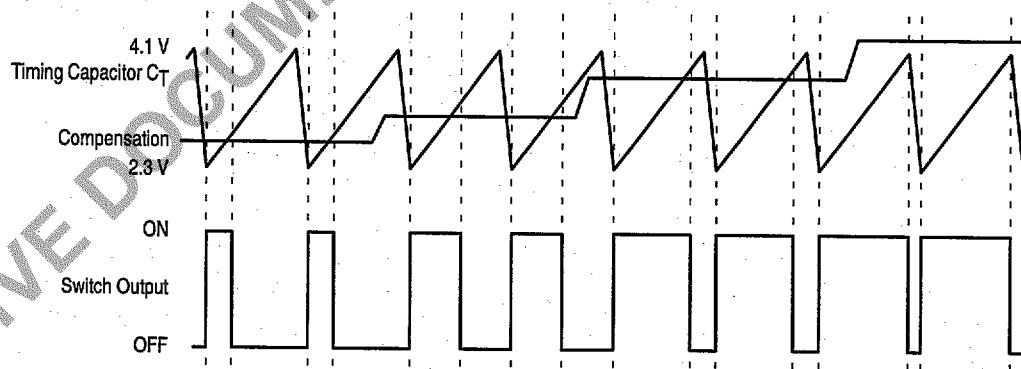
Figure 14. Timing Diagram
