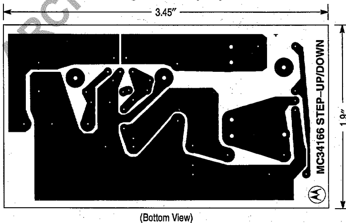
Figure 21. Step-Up/Down Converter Printed Circuit Board and Component Layout
