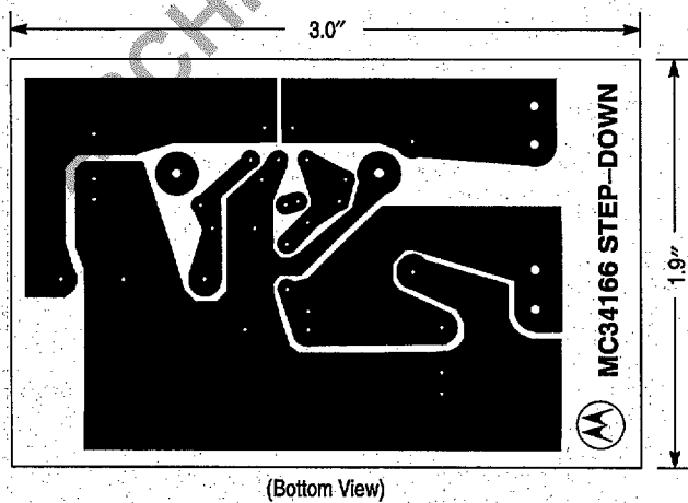
Figure 19. Step-Down Converter Printed Circuit Board and Component Layout
