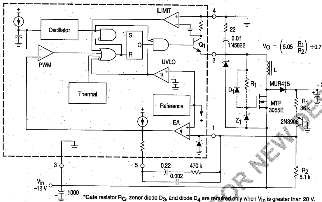
Figure 25. Negative Input/Positive Output Regulator
