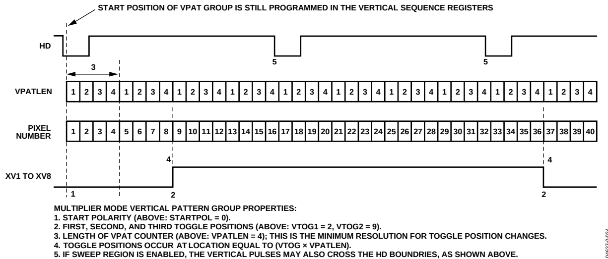
Figure 41. Example of Multiplier Region for Wide Vertical Pulse Timing
