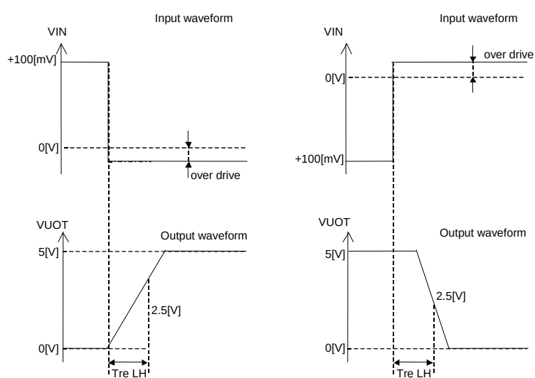
Fig.90 Response Time
