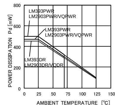
LM393DR/PWR/DGKR LM2903DR/PWR/DGKR/VQDR/VQPWR
