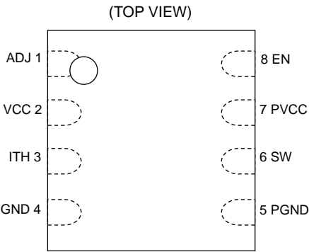
Figure 2. Pin Configuration
