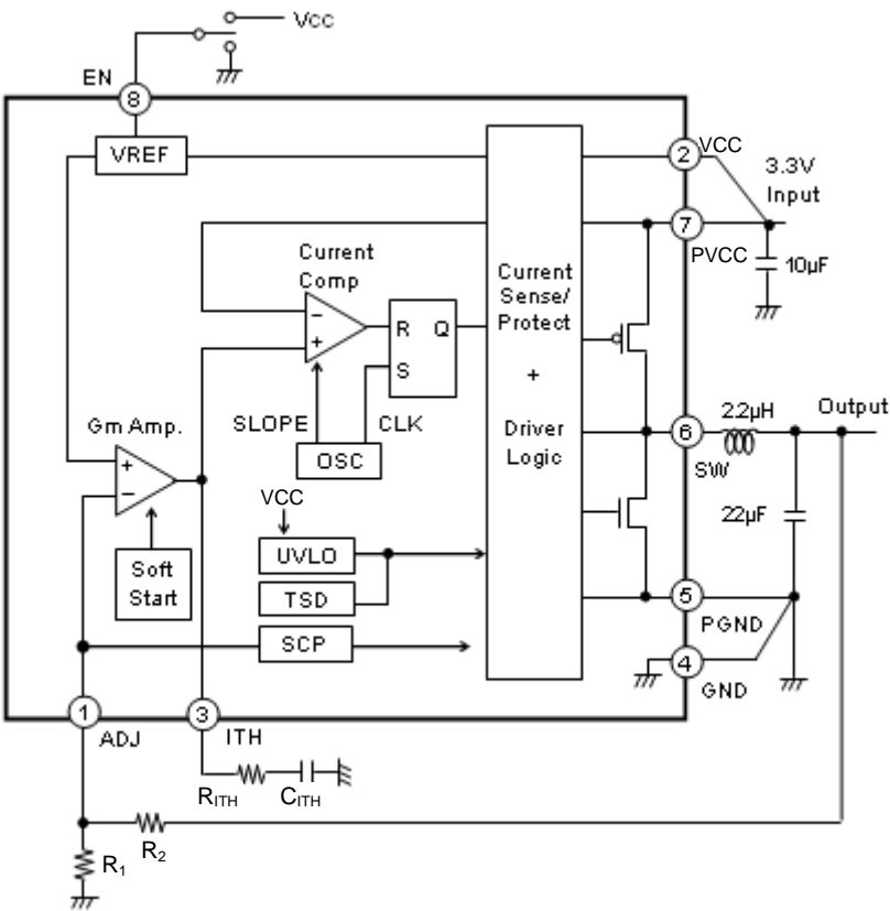
Figure 3. Block Diagram
