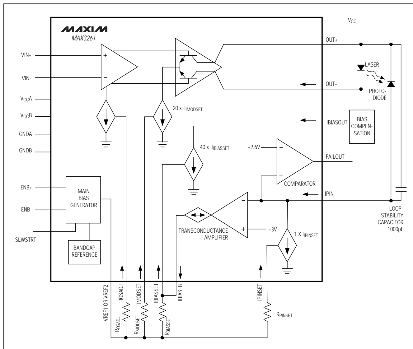
Figure 1. Functional Diagram
