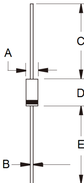
DO-204AC (DO-15)
