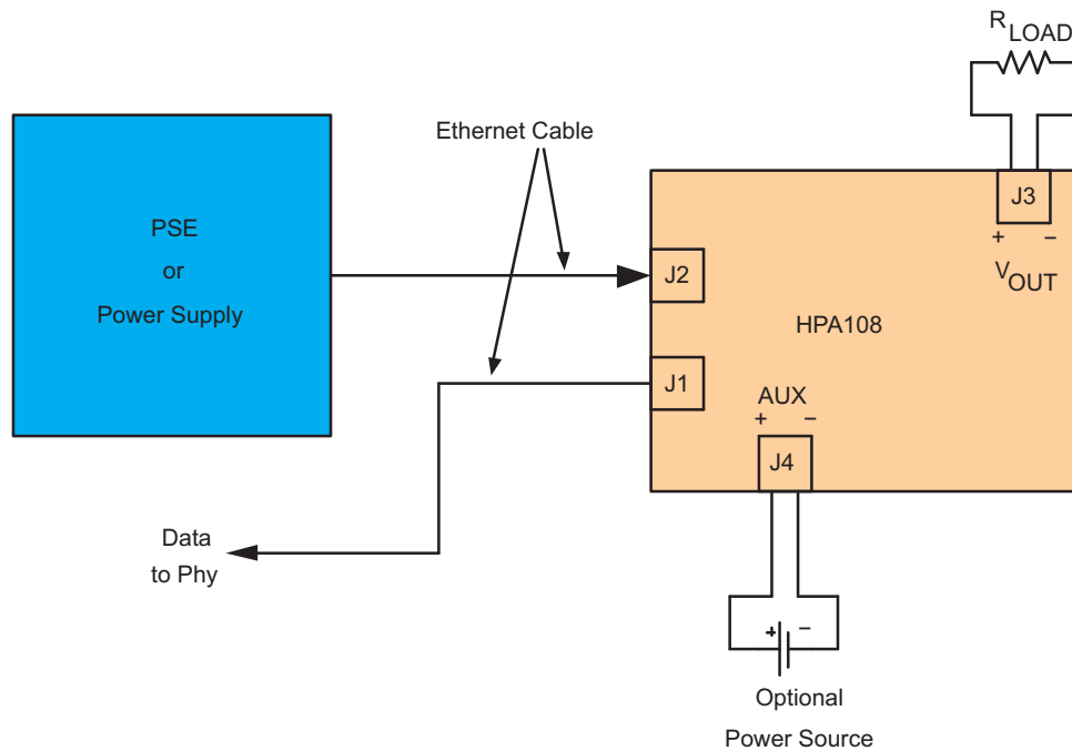
Figure 5. Typical Setup
