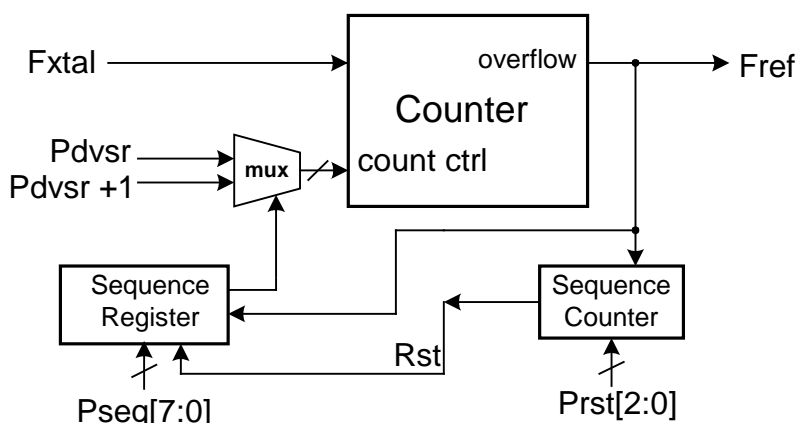
Figure 17: NCO Block Diagram
