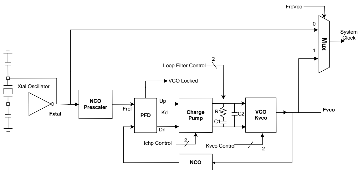
Figure 5: Clock Generation
