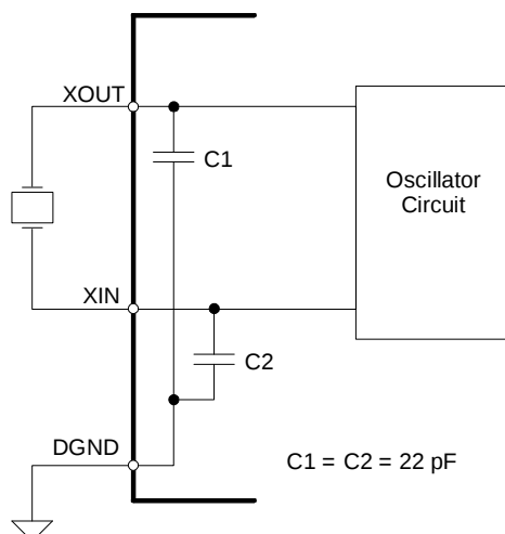
Figure 8. Oscillator Connection
