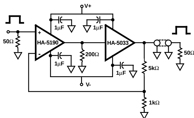
FIGURE 6. VIDEO PULSE AMPLIFIER COAXIAL LINE DRIVER
