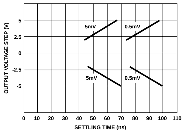
FIGURE 14. SETTLING TIME FOR VARIOUS OUTPUT STEP VOLTAGES
