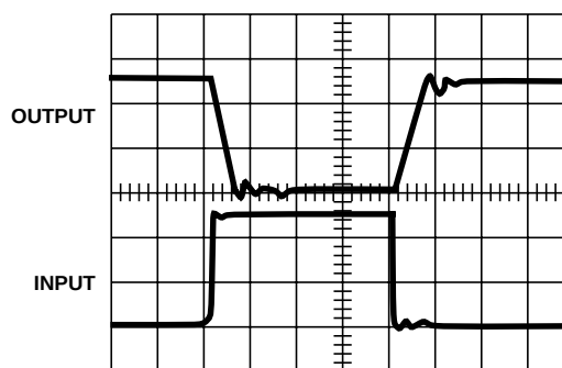
FIGURE 4. SUGGESTED COMPENSATION FOR INVERTING UNITY GAIN AMPLIFIER
