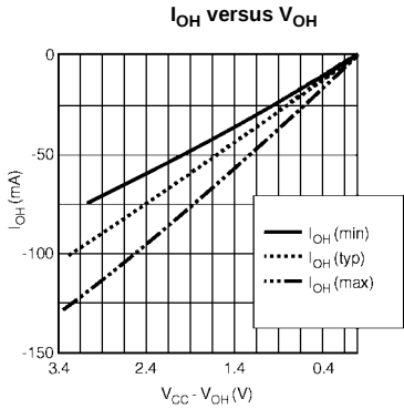
FIGURE 1. Characteristics for Output - Pull Up Drive
