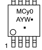
Micro8 MC34164DM CASE 846A
