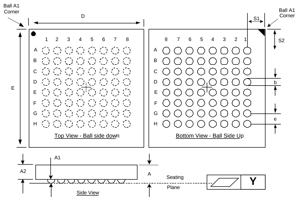
Figure 4: Easy BGA Package Drawing and Dimension
