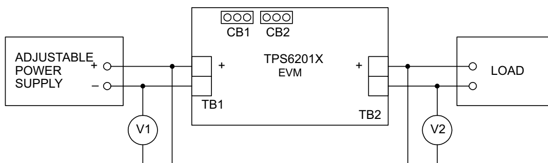
Figure 3-3. Connection Diagram
