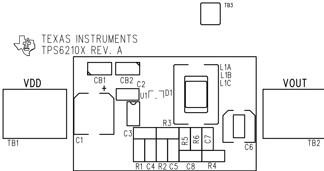
Figure 5-3. Assenmbly Drawing (Top Assembly)
