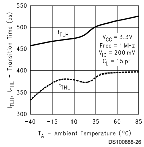
Transition Time vs Ambient Temperature
