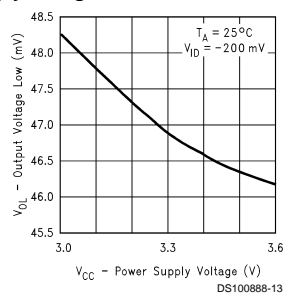
Output Low Voltage vs Power Supply Voltage
