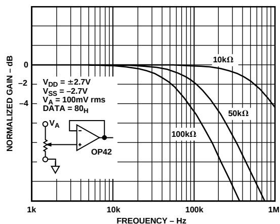
Figure 7. -3 dB Bandwidth vs. Terminal Resistance, \pm 2.7 V Dual Supply Operation
