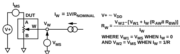
Figure 24. Wiper Resistance Test Circuit
