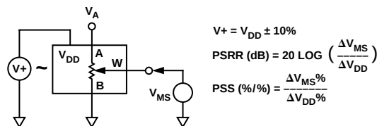
Figure 25. Power Supply Sensitivity Test Circuit (PSS, PSRR)
