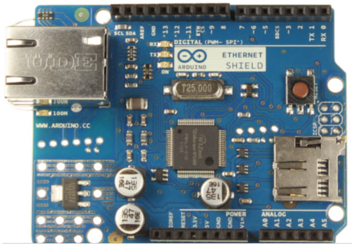
Arduino Ethernet Shield R3 Front
