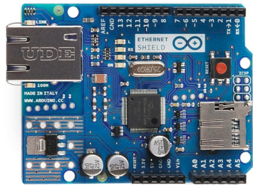
Arduino Ethernet Shield
