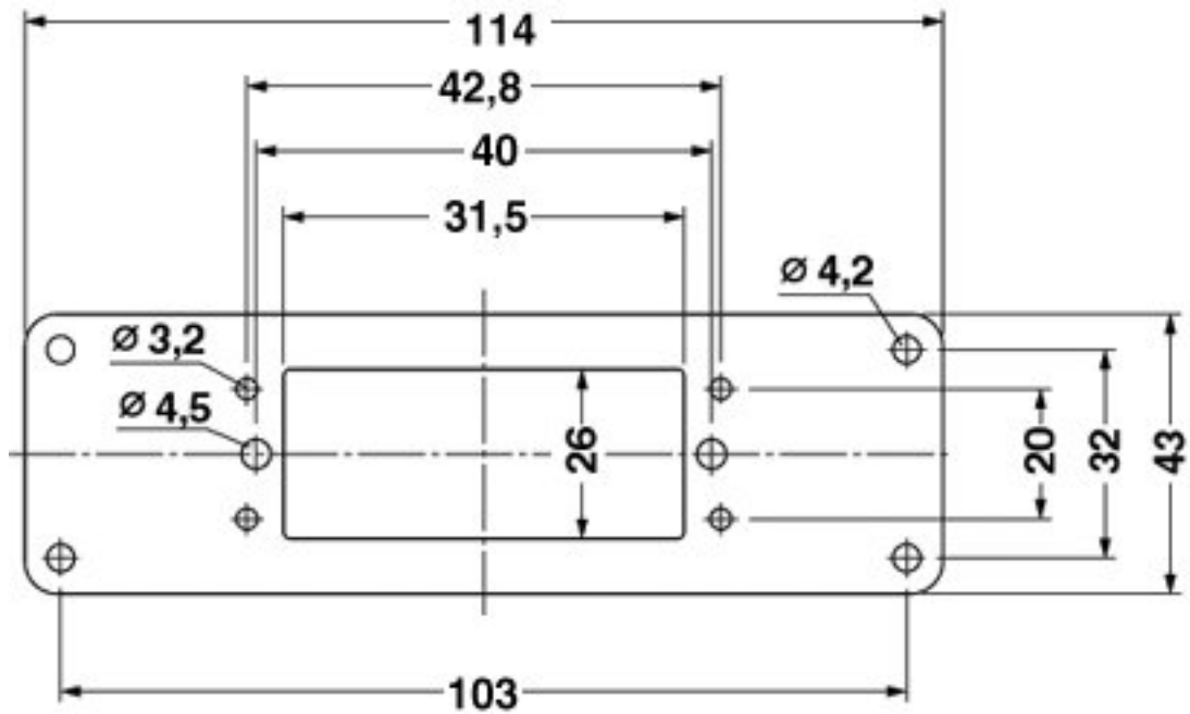
Dimensioned drawing
