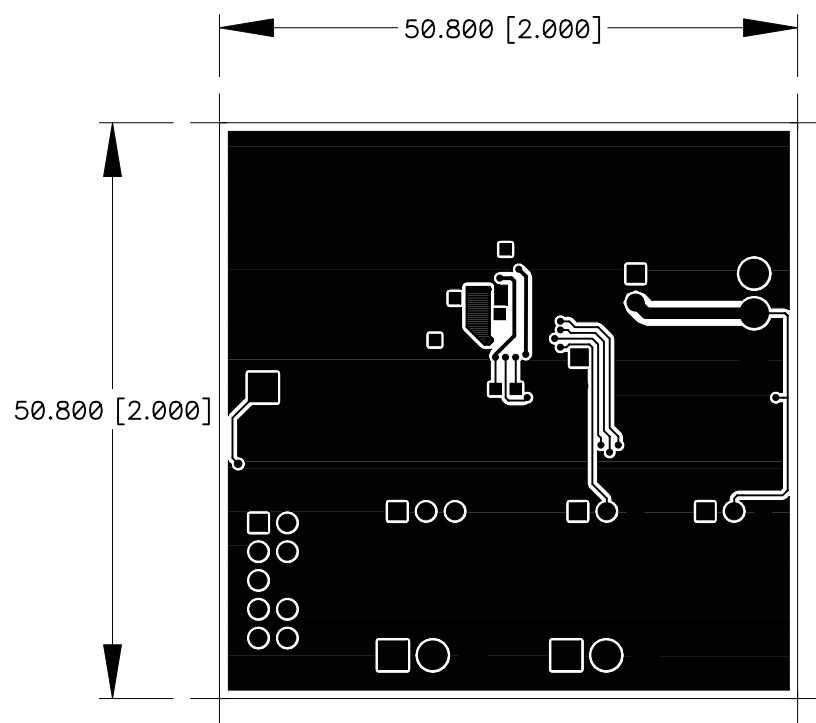
Figure 6. Bottom Layer
