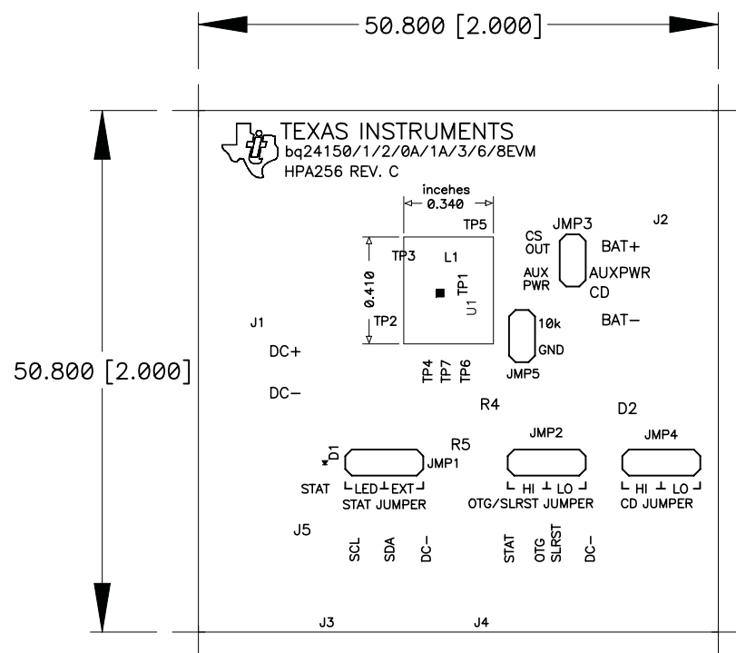
Figure 8. Top Silk
