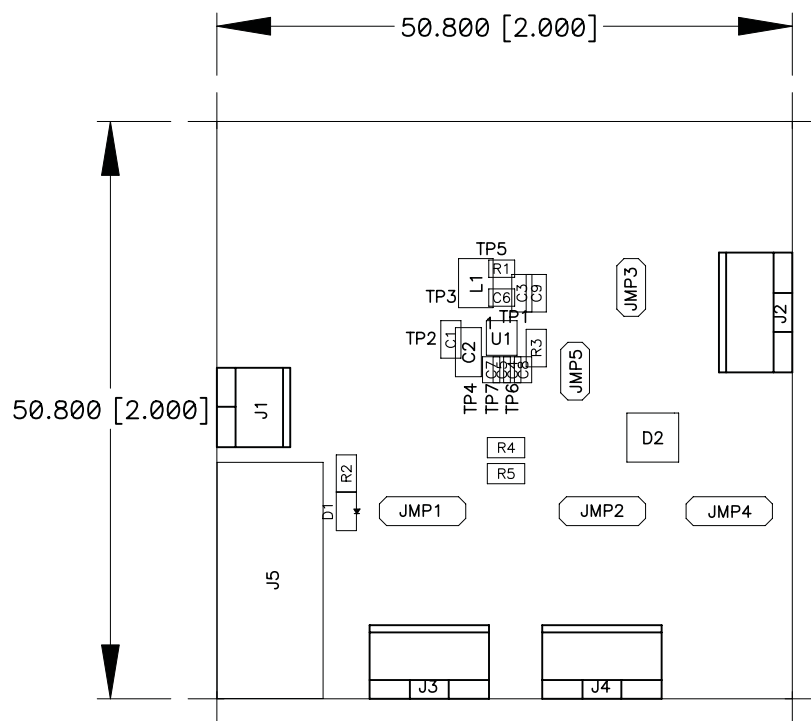
Figure 7. Top Assembly
