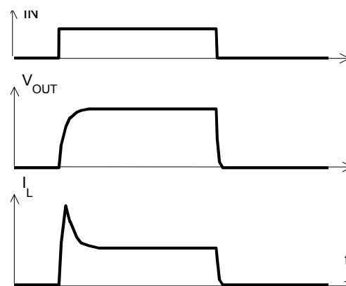
Figure 2b: Switching a lamp,
