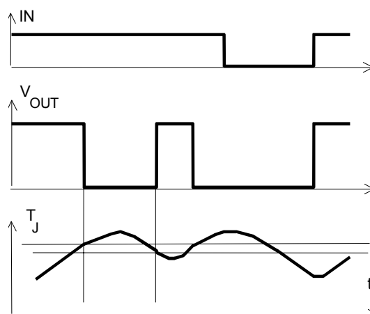
Figure 4a: Overtemperature: Reset if T_j < T_{jt}
