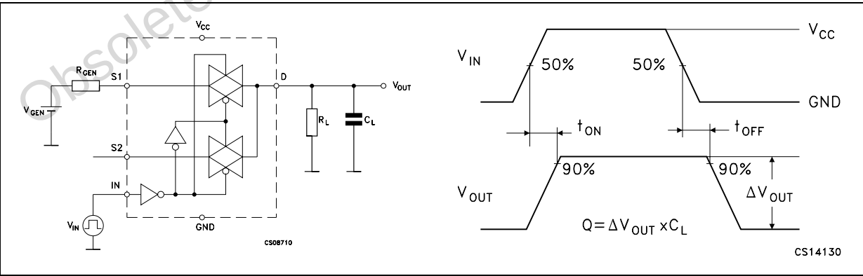
Figure 10: Charge Injection ( V_{GEN}=0\text{V} , R_{GEN}=0\Omega , R_L=1\text{M}\Omega , C_L=100\text{pF} )
