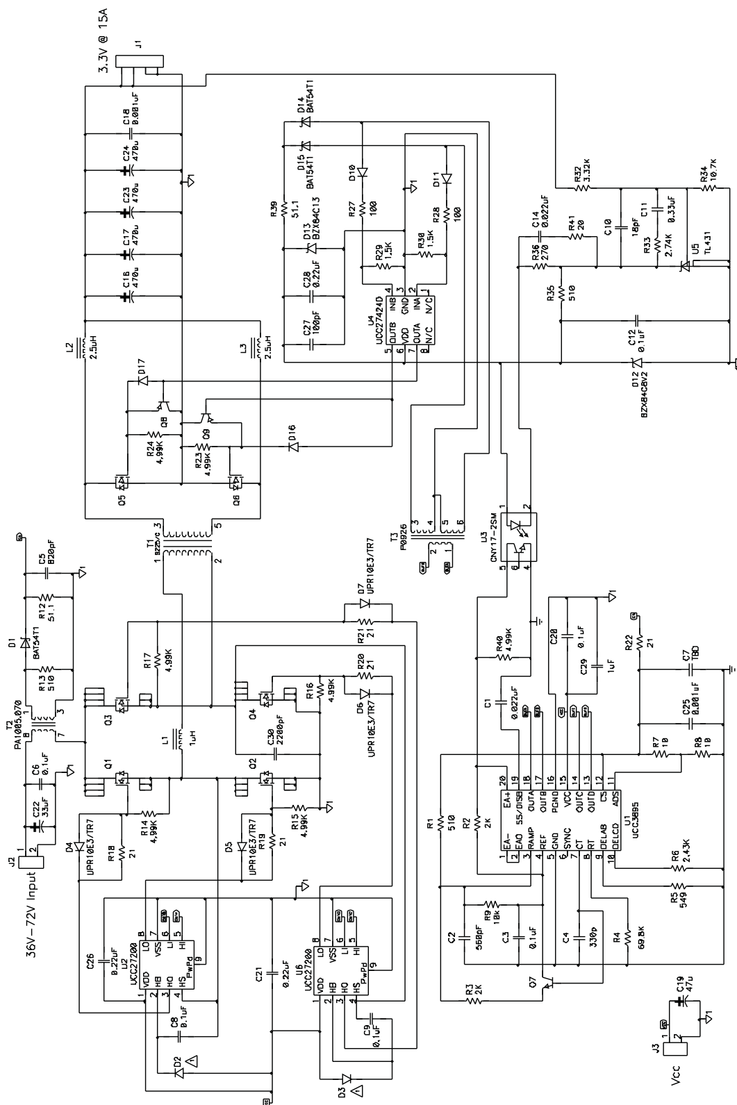
Figure 1. UCC3985EVM-001 Schematic
