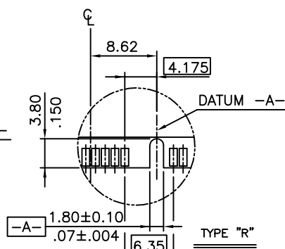
RECOMMENDED MODULE LAYOUT
