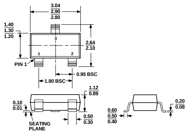
Figure 25. Surface-Mount Package [SOT-23]
