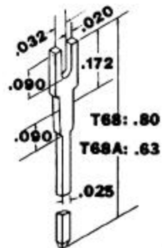
T68 SERIES MINIWRAP TERMINAL
