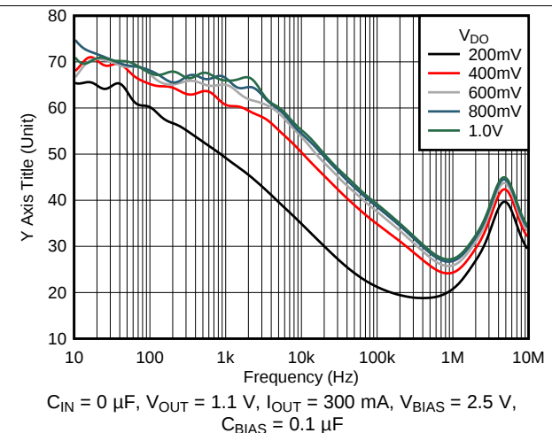
Figure 29. PSRR vs Frequency and V_{DO}
