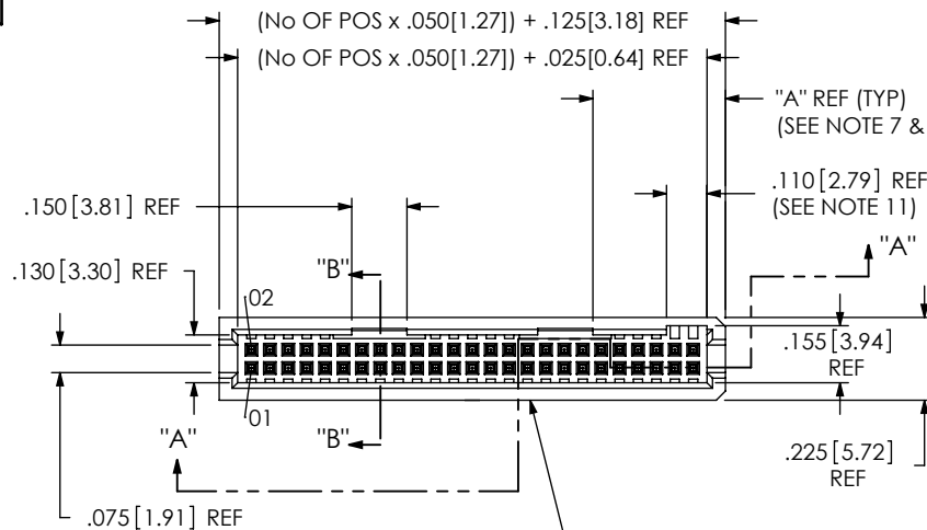
FIG 1 -01: THROUGH HOLE
