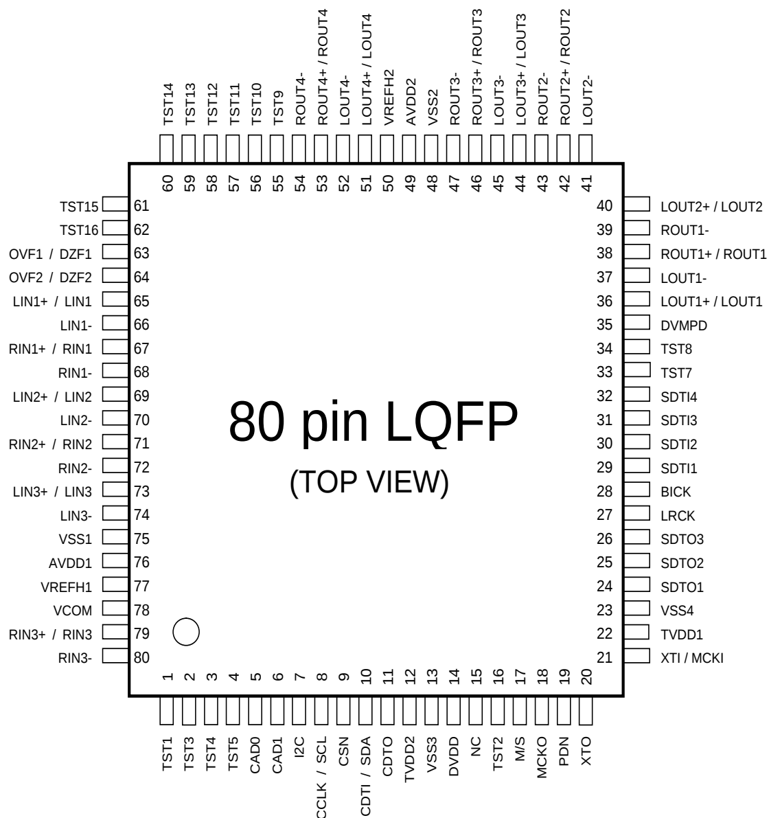
Figure 2. Pin Layout
