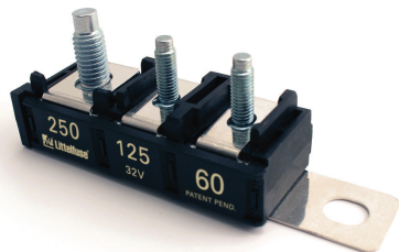
ZCASE Masterfuses
