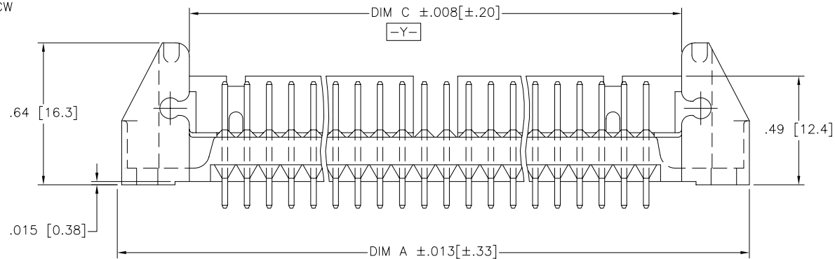
VIEW C-C
