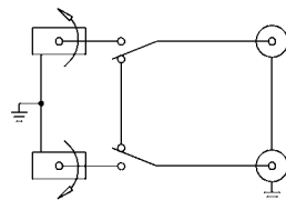
NORMALLED NON-TERMINATED
