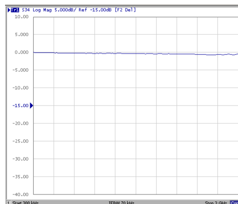
VJHD75TZ TYPICAL INSERTION LOSS
