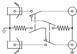
NON-NORMALLED TERMINATED
