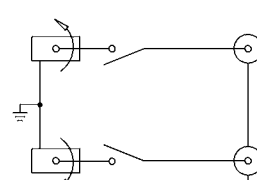
NON-NORMALLED NON-TERMINATED
