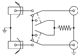
NORMALLED TERMINATED
