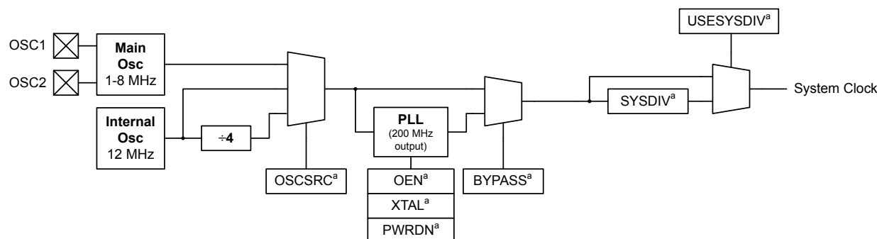
Figure 6-4. Main Clock Tree
