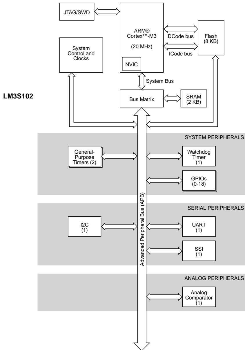
Figure 1-1. Stellaris® LM3S102 Microcontroller High-Level Block Diagram
