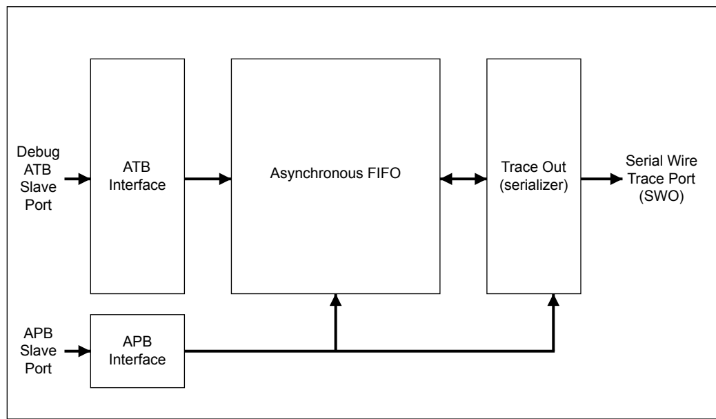
Figure 2-2. TPIU Block Diagram
