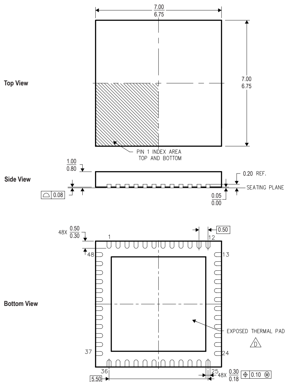
Figure D-3. 48-Pin QFN Package
