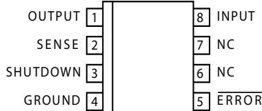
MIC29201-3.3BM (SOIC-8)
