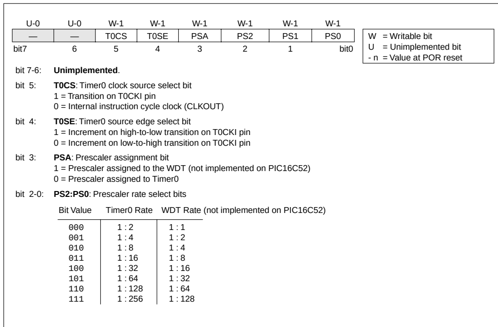
FIGURE 4-9: OPTION REGISTER
