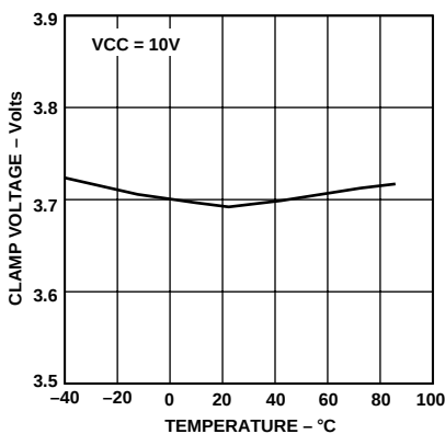
Figure 17. DRV Output Low Voltage with VCC = 10 V vs. Temperature
