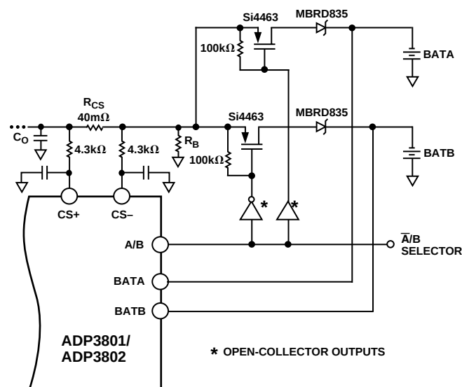
Figure 31. Dual Li-Ion Battery Charger
