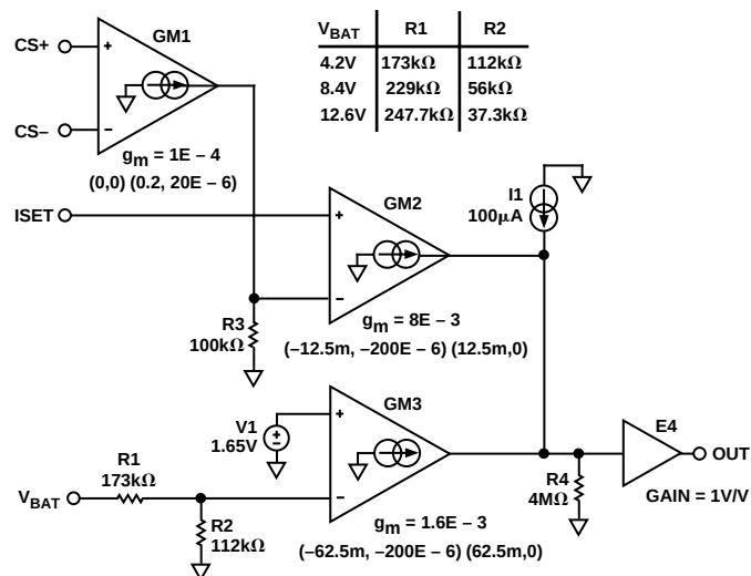
Figure 29. AC Behavioral SPICE Model for the ADP3801 and ADP3802
