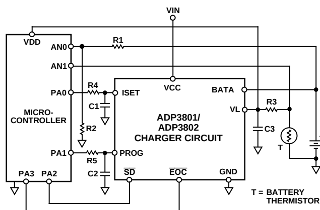
Figure 30. Universal Battery Charger Block Diagram
