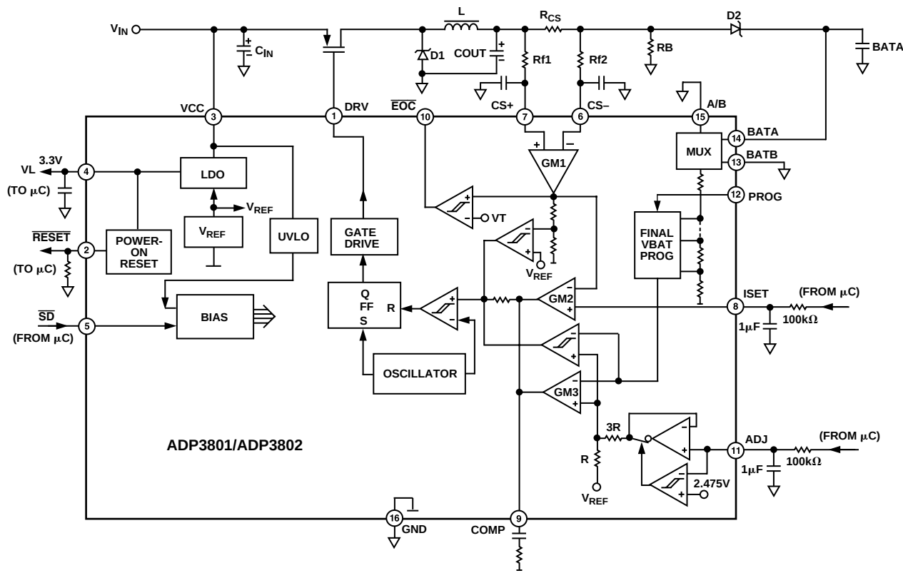
Figure 20. Simplified Application Diagram
