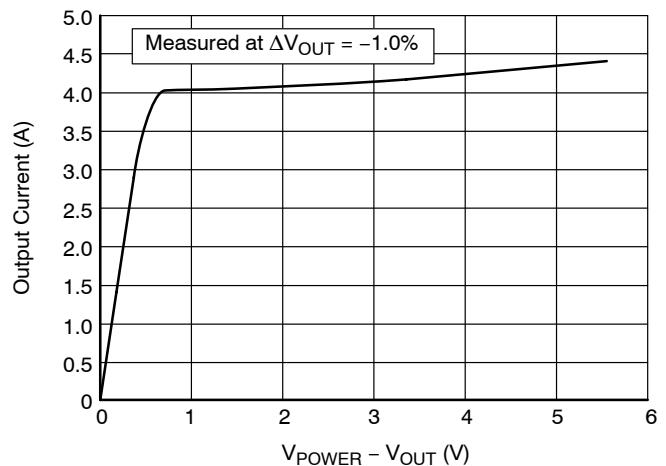
Figure 6. Output Current vs V_{\text{POWER}} - V_{\text{OUT}}
