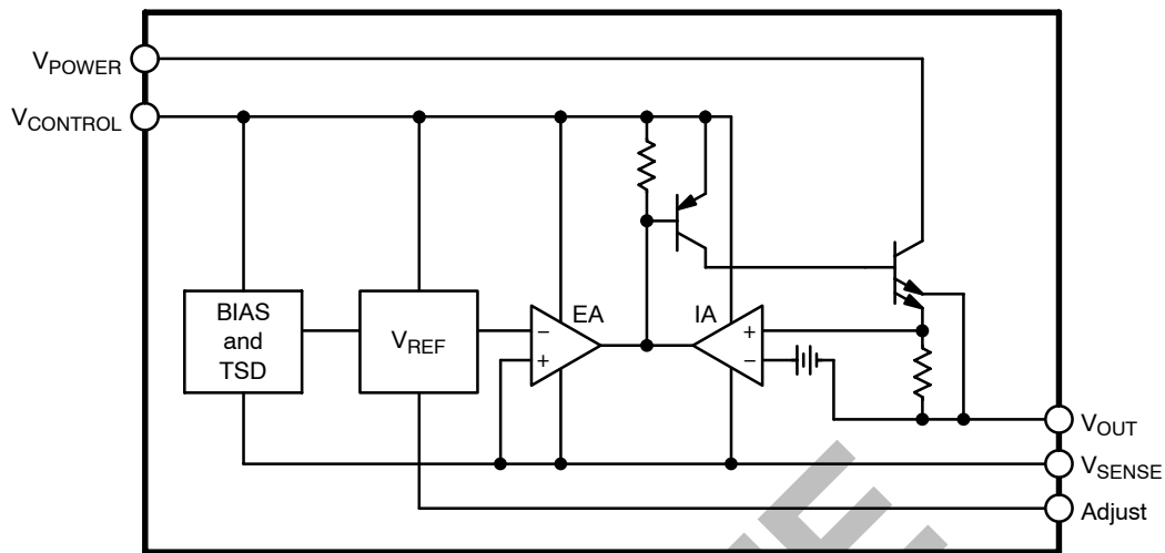
Figure 2. Block Diagram
