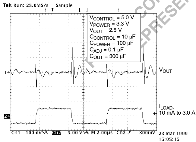
Figure 5. Transient Response
