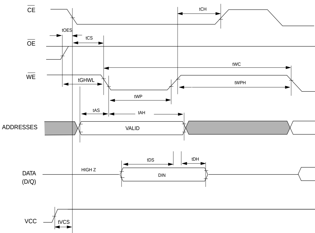
Figure 7. COMMAND WRITE TIMING WAVEFORMS
