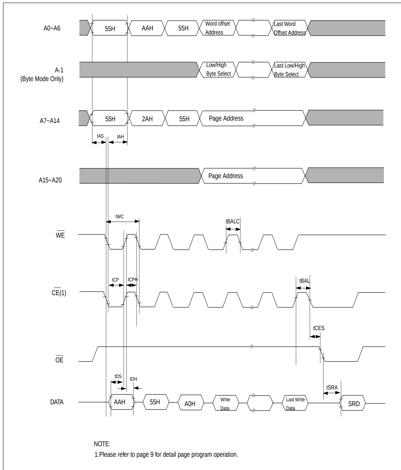
Figure 14. AUTOMATIC PAGE PROGRAM TIMING WAVEFORM(Alternate \overline{\text{CE}} Controlled)
